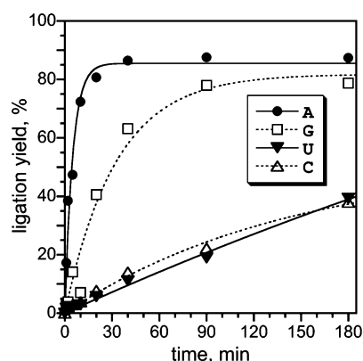
FIGURE 4: Branched RNA formation by the 10DM24 deoxyribozyme shows a clear preference for branch-site adenosine. k_{\text{obs}} values ( \pm standard error of the mean; n = 3 in each case): 0.26 \pm 0.02 \text{ min}^{-1} for A, 0.035 \pm 0.002 \text{ min}^{-1} for G, 0.0035 \pm 0.0011 \text{ min}^{-1} for U, and 0.0030 \pm 0.0007 \text{ min}^{-1} for C ( k_{\text{A}}/k_{\text{U}} = 73 ). For comparison, 7S11 synthesizes A-branched RNA with a k_{\text{obs}} of \approx 0.5 \text{ min}^{-1} and a k_{\text{A}}/k_{\text{U}} of \approx 3000 (3, 4). See Table 1 for similar data for all new deoxyribozymes.
